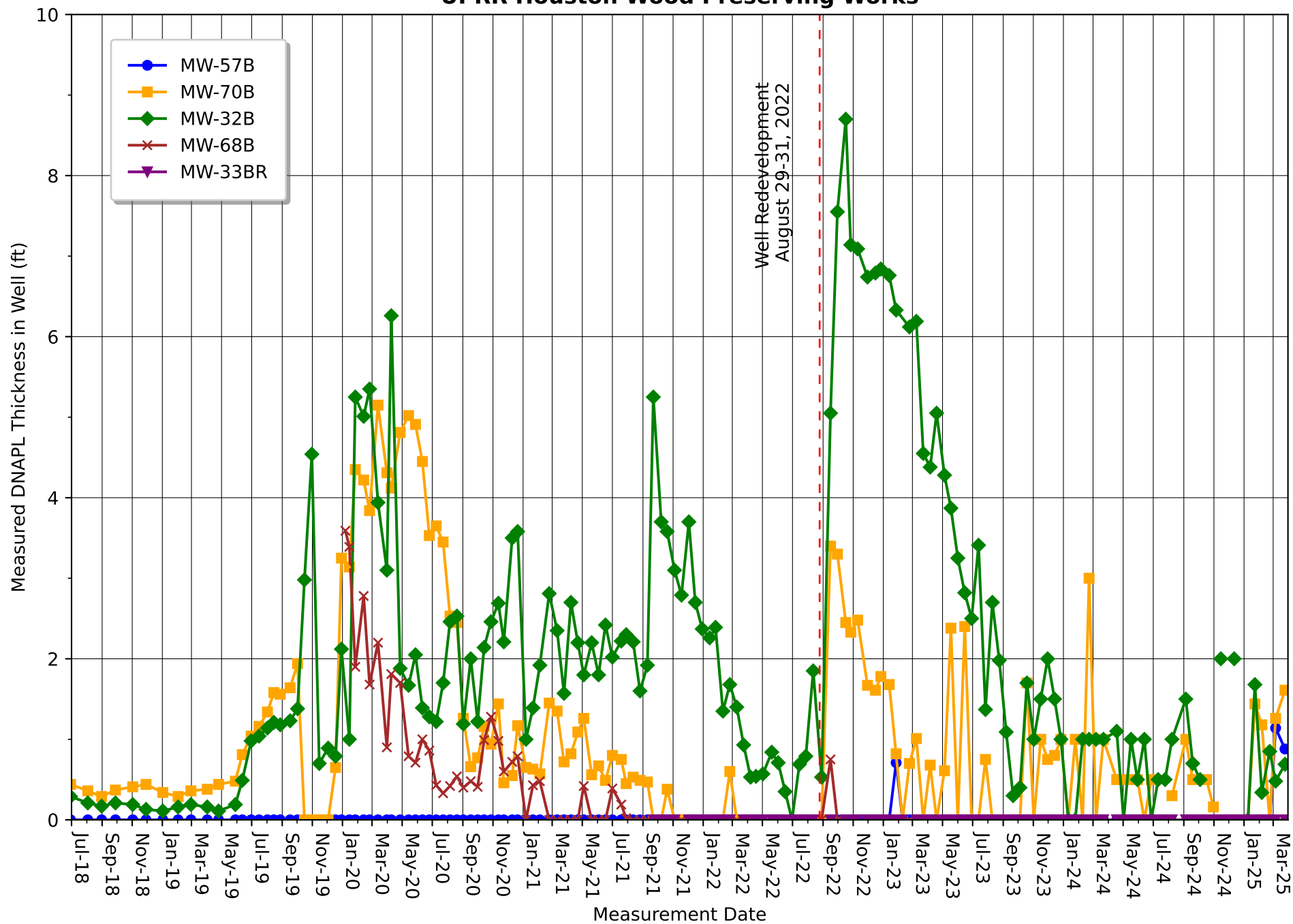
Figure 5 B-CZ/B-TZ Wells (North (On-site and Off-site)-DNAPL Recovery Activities July 2018 - March 2025 UPRR Houston Wood Preserving Works
