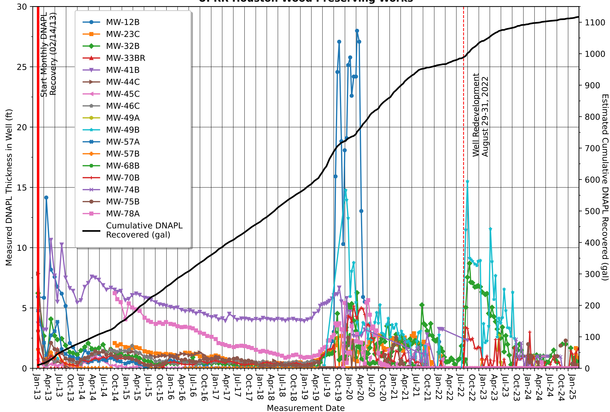
Figure 2 DNAPL Recovery Activities February 2013 - March 2025 UPRR Houston Wood Preserving Works
