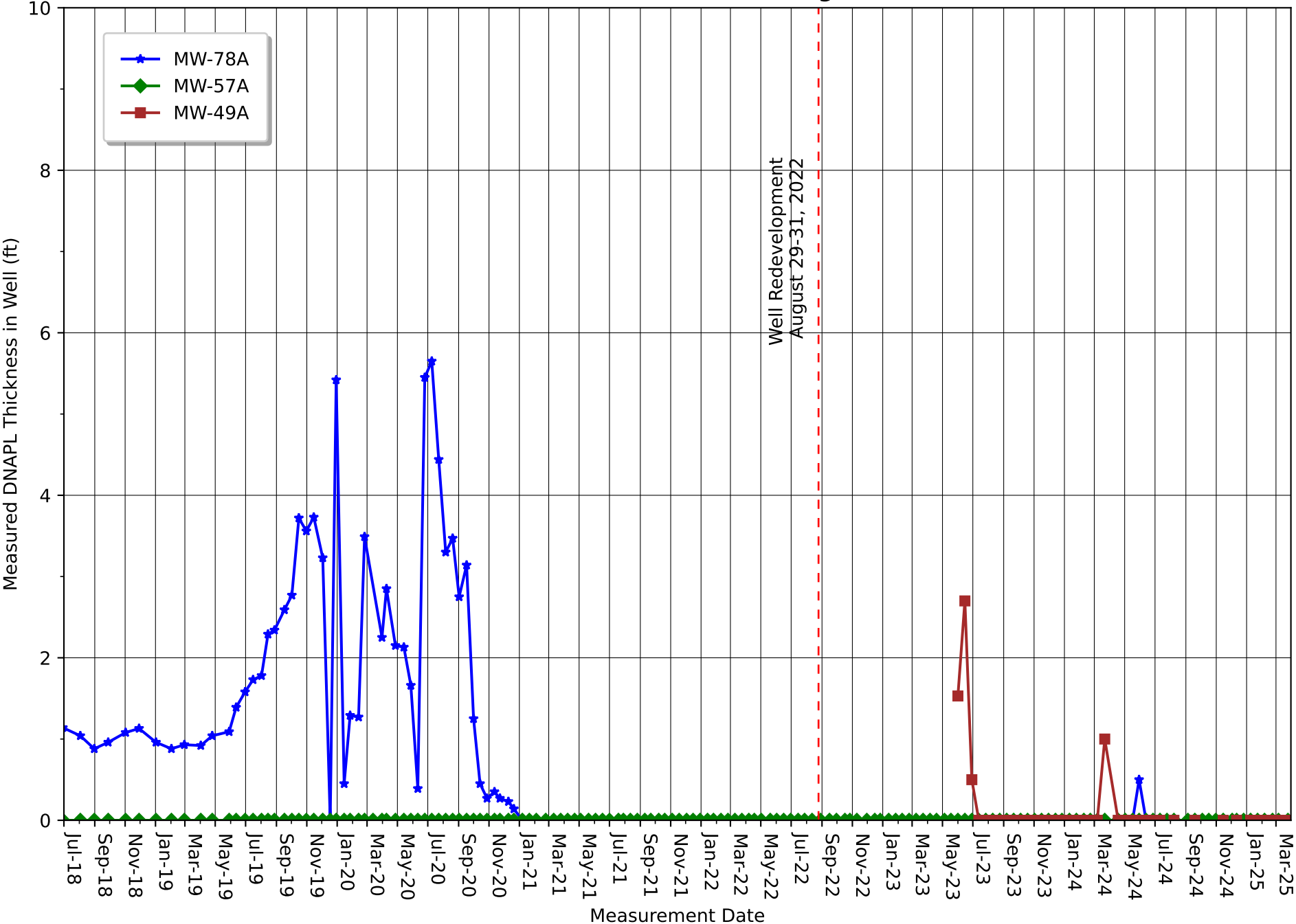
Figure 3 A-TZ Wells-DNAPL Recovery Activities July 2018 - March 2025 UPRR Houston Wood Preserving Works
