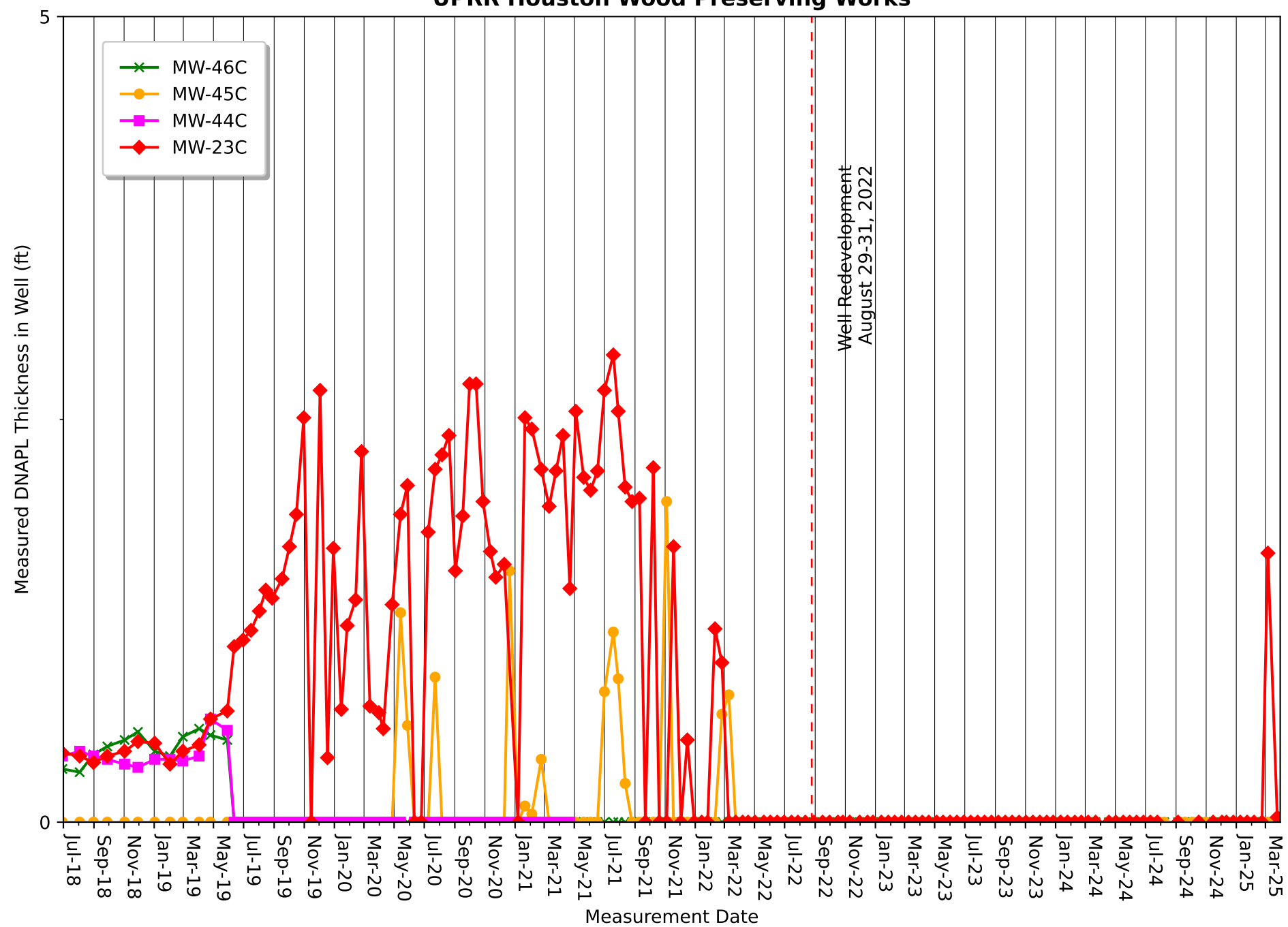
Figure 7 C-TZ Wells-DNAPL Recovery Activities July 2018 - March 2025 UPRR Houston Wood Preserving Works
