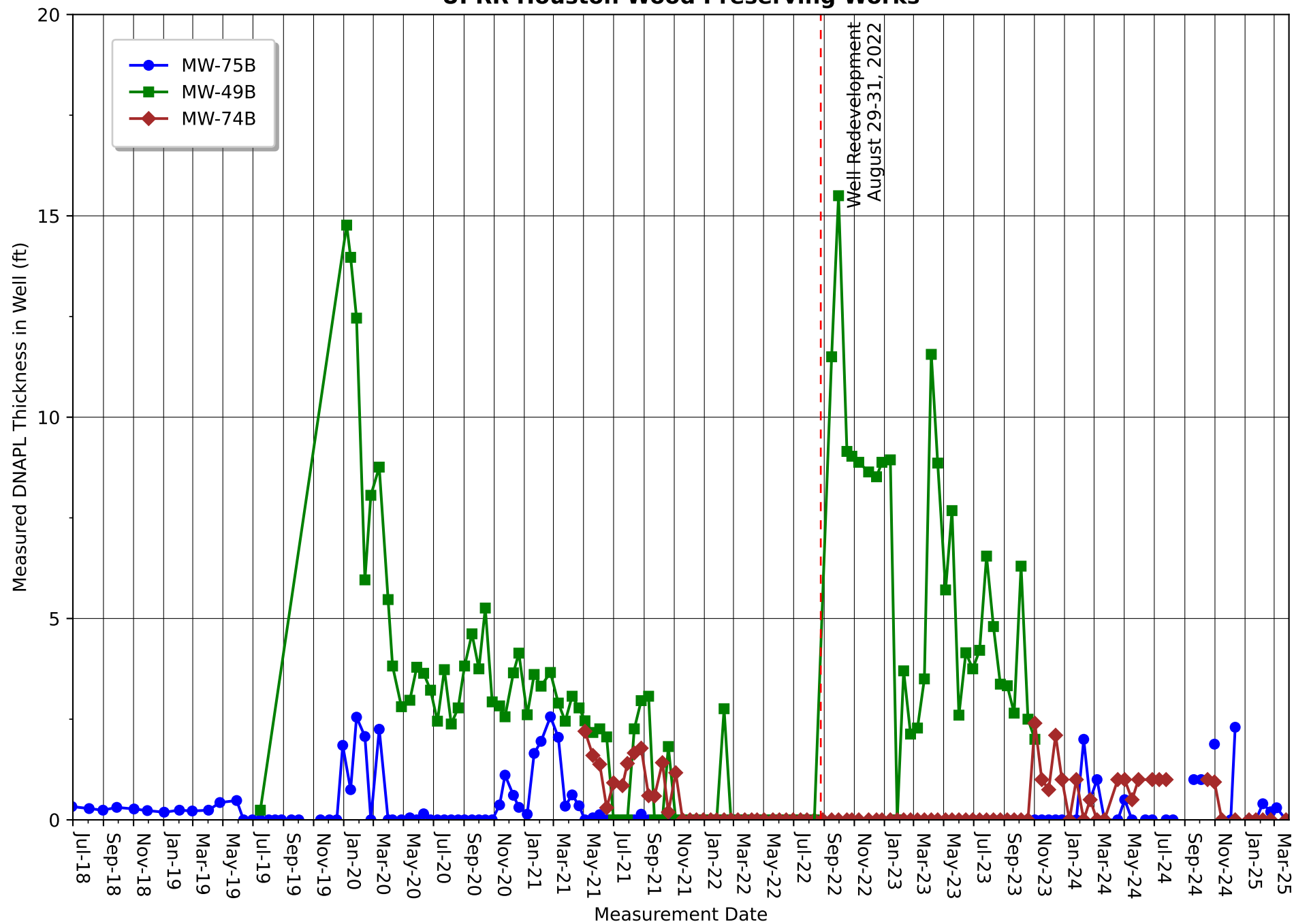
Figure 6 B-CZ/B-TZ Wells (Englewood Intermodal Yard)-DNAPL Recovery Activities July 2018 - March 2025 UPRR Houston Wood Preserving Works
