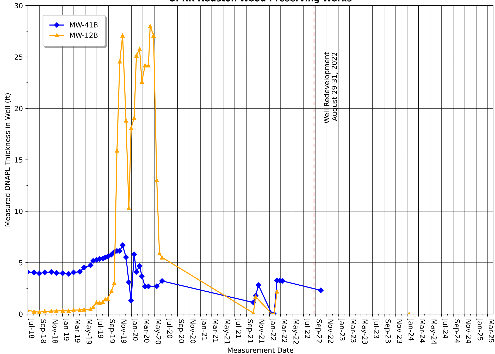
Figure 4 B-TZ Wells (West Side)-DNAPL Recovery Activities July 2018 - March 2025 UPRR Houston Wood Preserving Works
