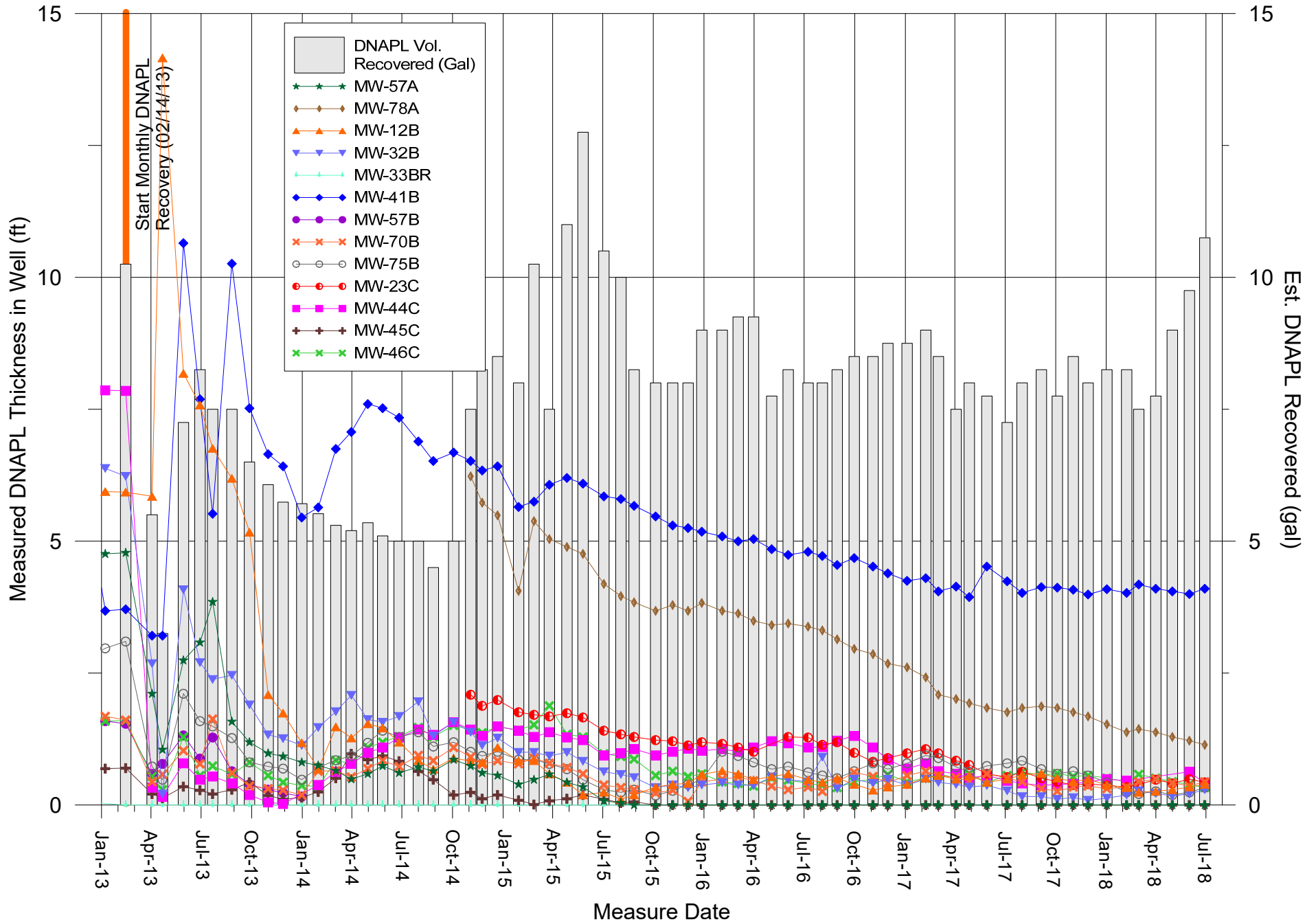
Figure 2 DNAPL Recovery Activities February 2013 - June 2018 UPRR Houston Wood Preserving Works
